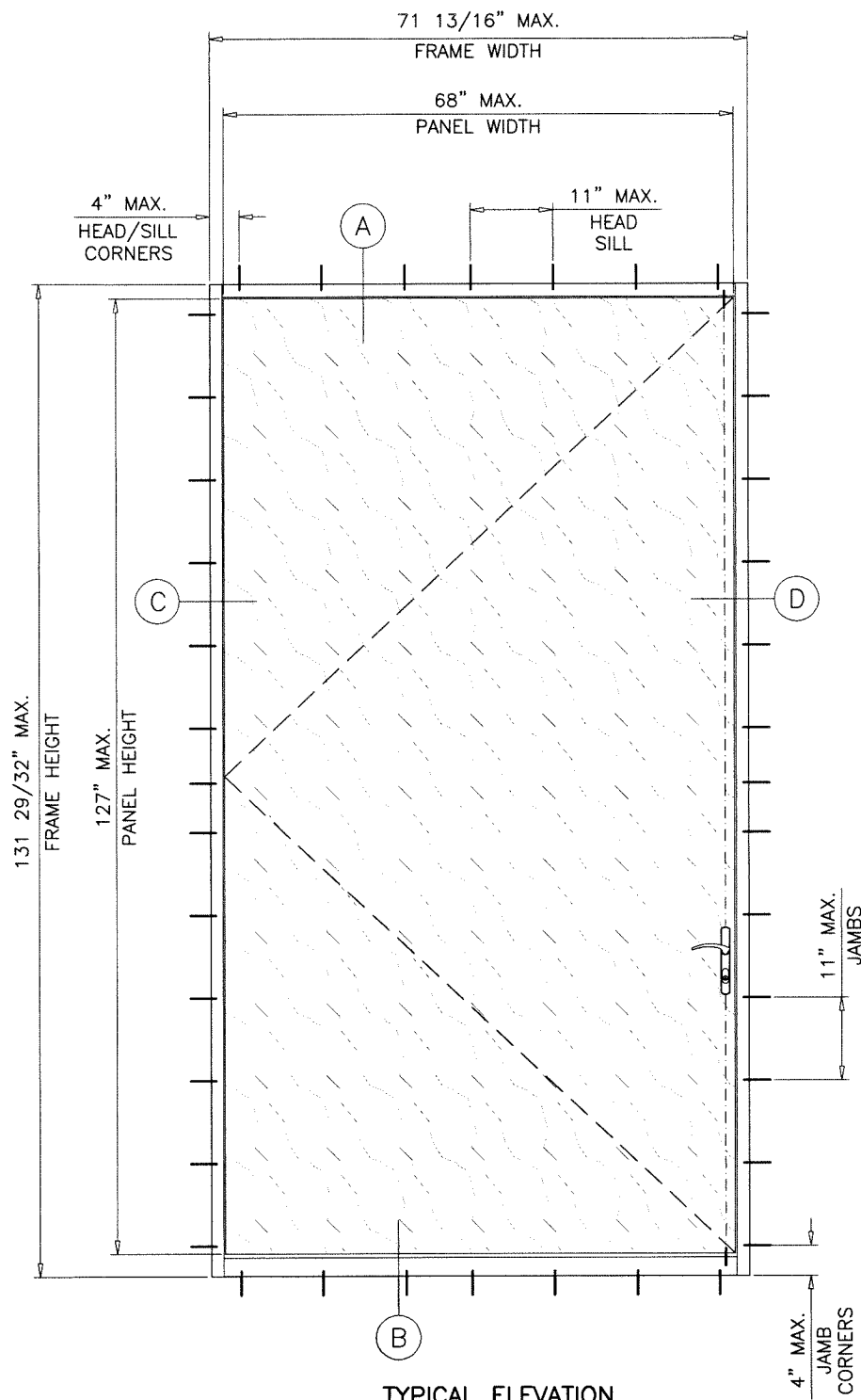
TYPICAL ELEVATION
